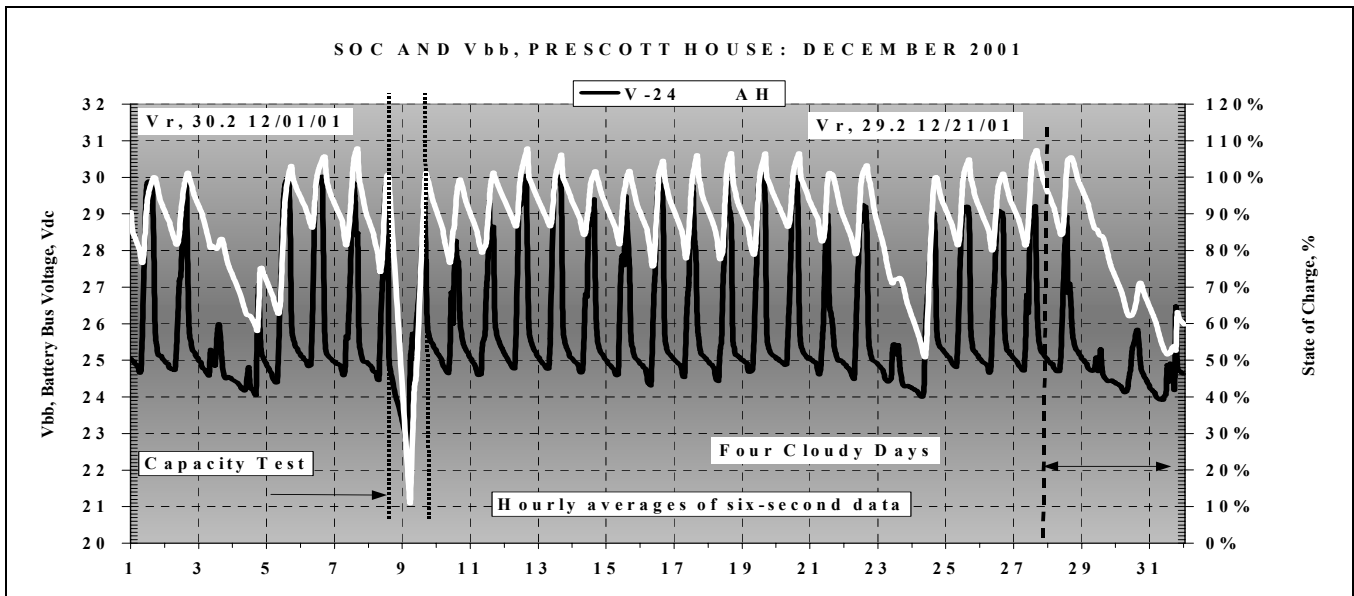
Figure 9. Battery Voltage and State of Charge for a residential PV system (December 2001)
