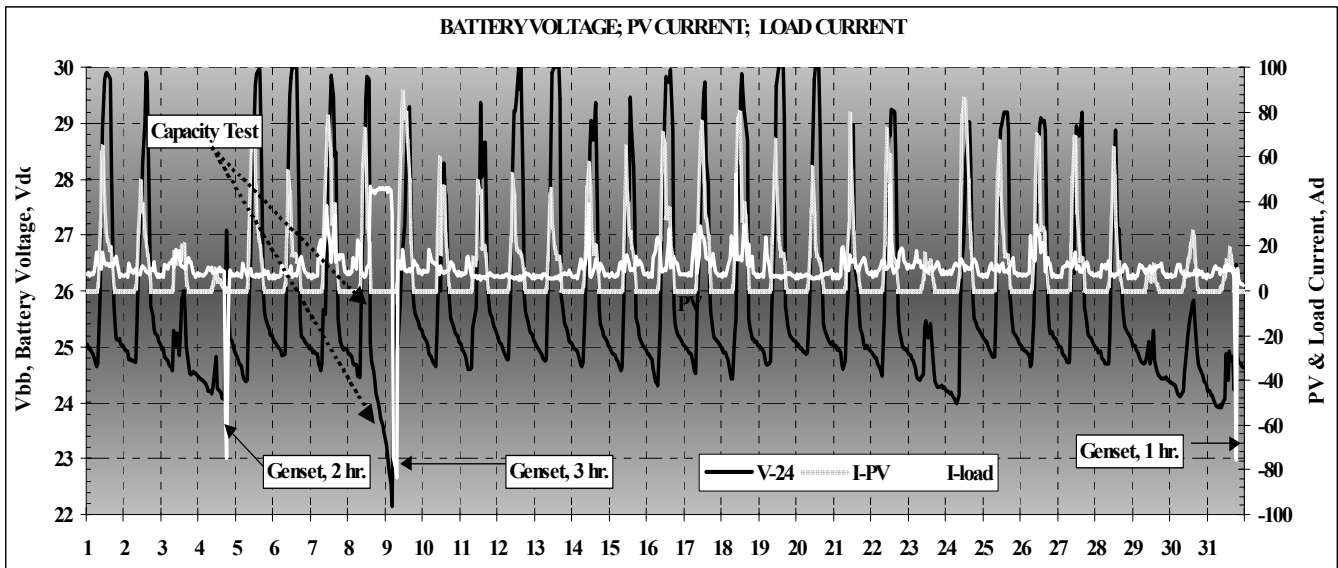
Figure 8. Battery Voltage, PV Current, and Load Current
