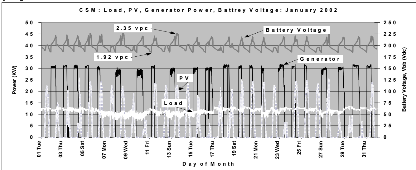
Figure 10. CSM Load KWH, PV KWH, Generator KWH, and Battery Voltage
