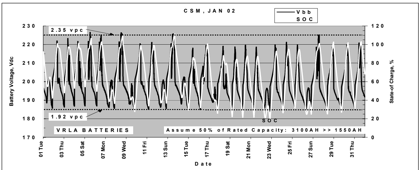
Figure 11. Battery Voltage and State-of-Charge for Carol Spring Mountain, January 2002
